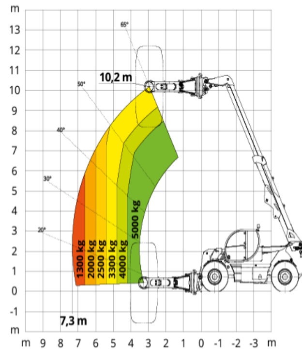
LOAD CHART WITH TYRES CLAMP MODEL TC 08.63
