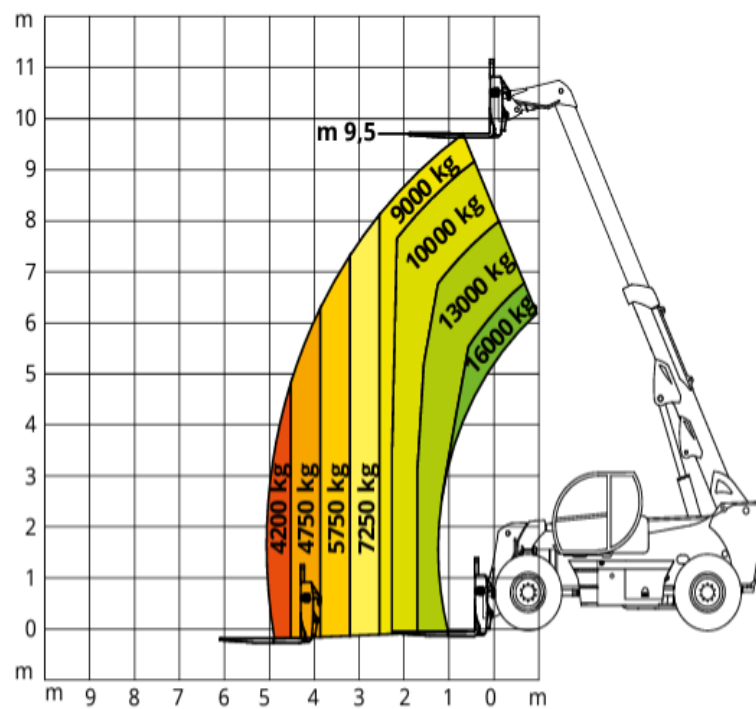
LOAD CHART WITH FORKS
